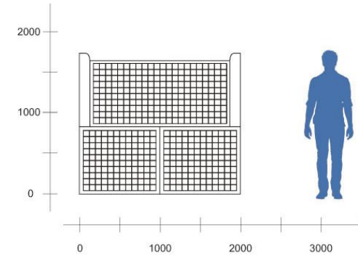
Rahmen (R) Inhalt ca. 3,4 m 3 ca. 1,00m x 1,80m x 2,00m (L x H x B)
